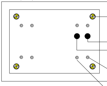
(A.10) CANOPY BOTTOM VIEW
